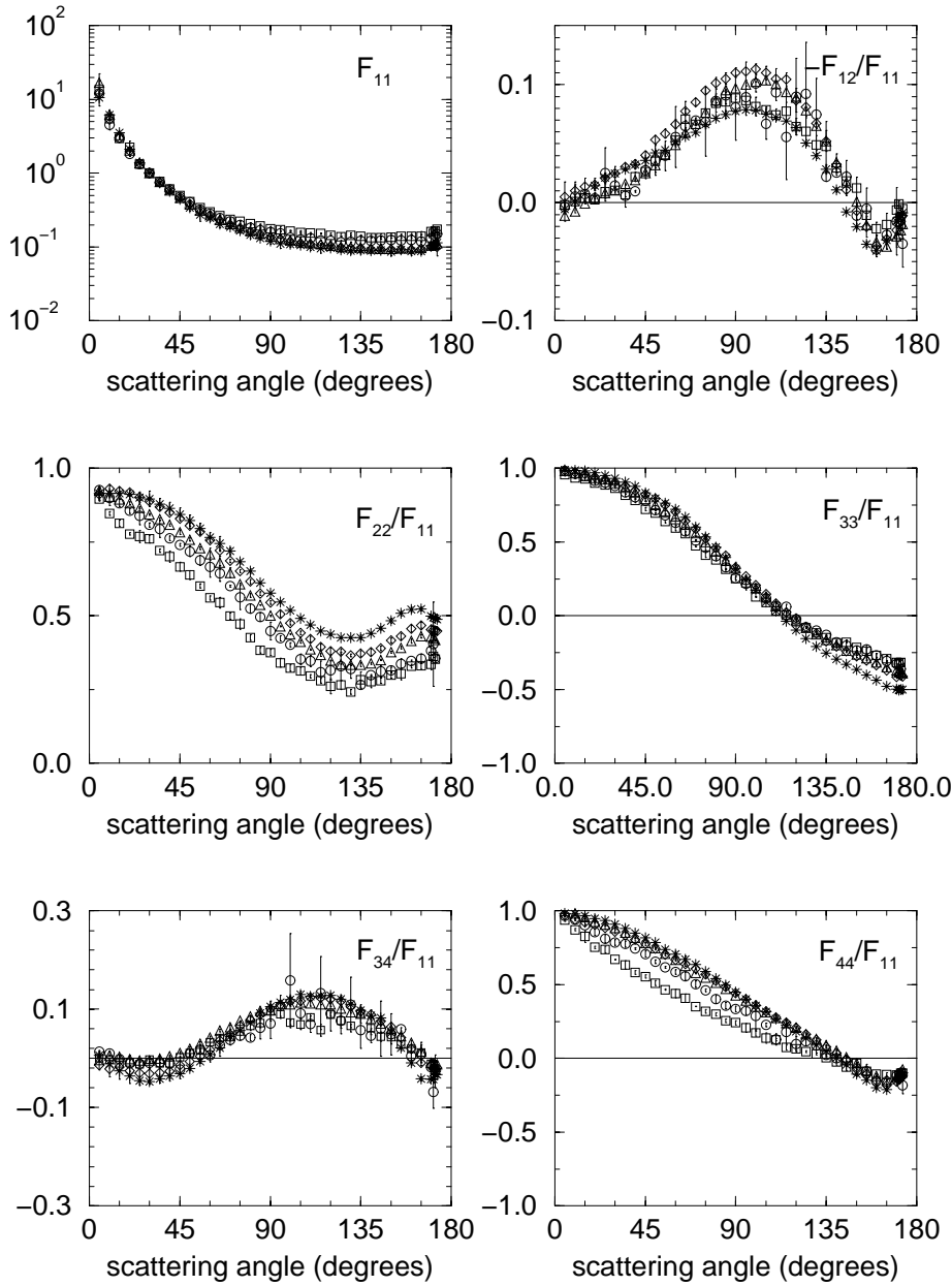
Fig. 6. Same as 5 but at 633 nm.
