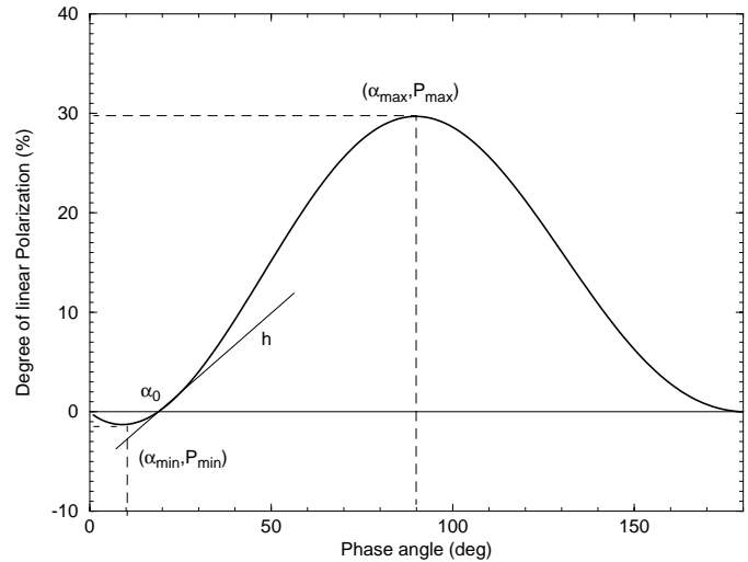
Fig. 8. Simulated typical polarization vs. phase curve for cometary or interplanetary dust particles (adapted from Levasseur-Regourd et al. 1999b).
