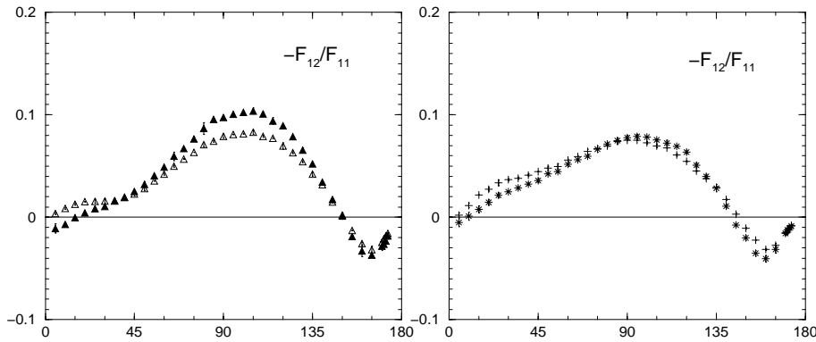
Fig. 7. Measured degree of linear polarization as function of scattering angle of olivine sample S (left panel) and Allende meteorite (right panel). Open triangles and pluses correspond to the results at 442 nm and filled triangles and stars to the results at 633 nm.
