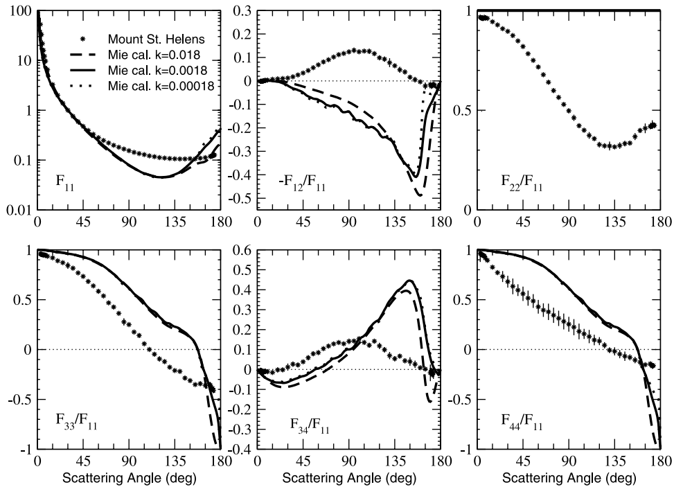
Figure 10. Measured scattering matrix elements as functions of the scattering angle at 632.8 nm for the Mount St. Helens sample. The measurements are presented together with results of Lorenz-Mie calculations for spheres with the same size distribution as the Mount St. Helens sample. For the calculations the real part of the refractive index was fixed at 1.5, and the imaginary part was varied between 0.018 (dashed lines), 0.0018 (solid lines), and 0.00018 (dotted lines).
