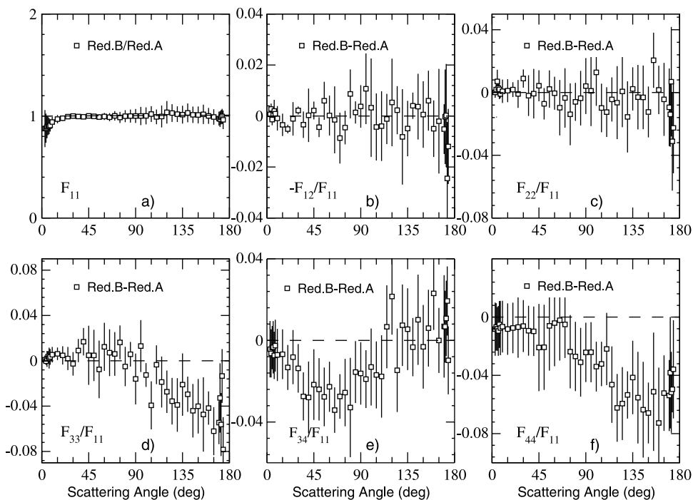
Figure 8. (a) Measured F_{11}(\theta) for Redoubt B divided by the measured F_{11}(\theta) for Redoubt A. (b–f) Differences between the indicated measured ratios for Redoubt B and Redoubt A.
