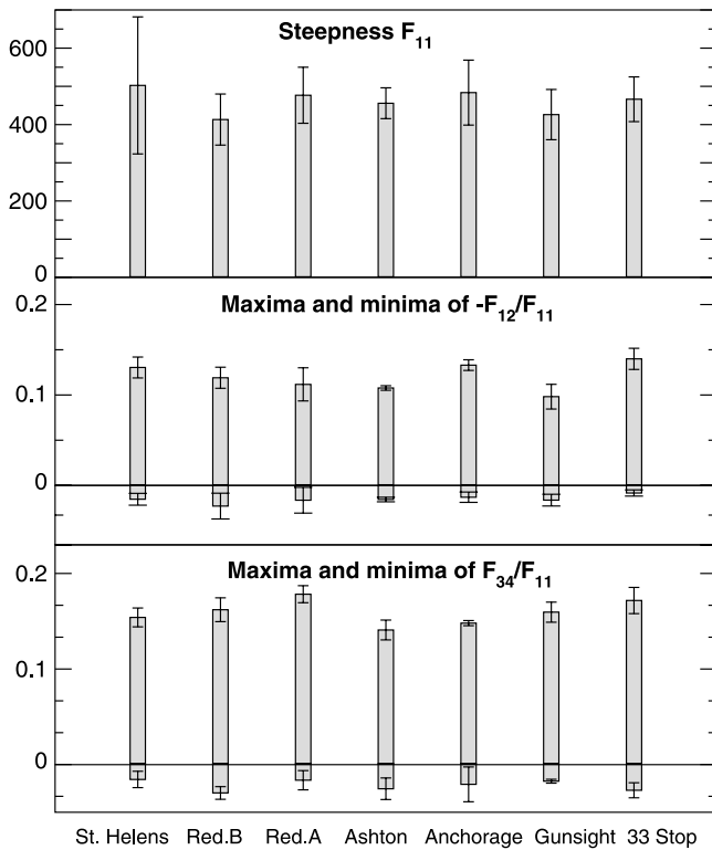
Figure 7. Properties of the measured scattering matrix elements. (top) Steepnesses of F_{11}(\theta) . (center) Maximum and minimum measured values of -F_{12}(\theta)/F_{11}(\theta) . (bottom) Maximum and minimum measured values of F_{34}(\theta)/F_{11}(\theta) . Error bars are also shown.
